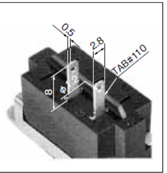
TAB 端子 #110 (ON-OFF)
